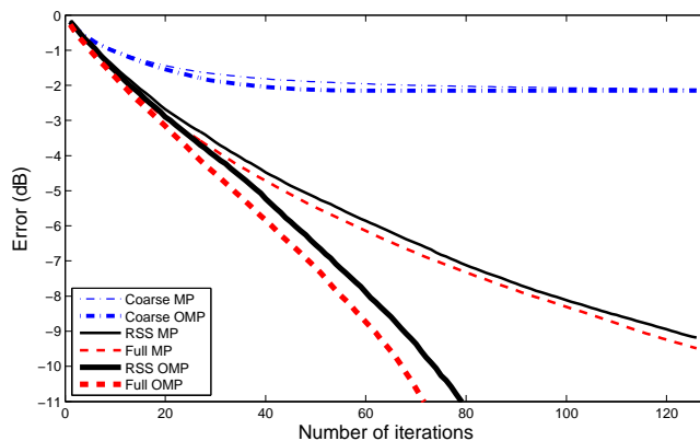
Figure 9: Comparison between algorithm MP (thin) and OMP (bold) with fixed coarse subdictionary \Phi_{\mathcal{T}_0} (dashed dotted blue), random sequential subdictionaries \Phi_{\mathcal{T}^n} and full dictionary \Phi (dashed red). Input signal is a collection of N/2 vectors from \Phi with normal weights. Results averaged over 1000 runs. Here N = 128 , M = 256
